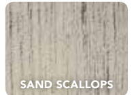
SAND SCALLOPS
